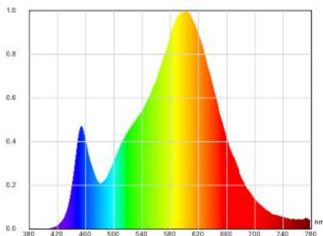
Spectrum Curve
