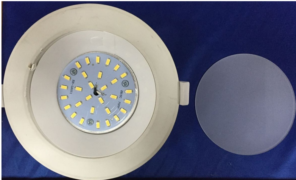
Picture 10. model: B0104-15-Y-1-Z, B0104-15-Y-3-Z internal view (I)
