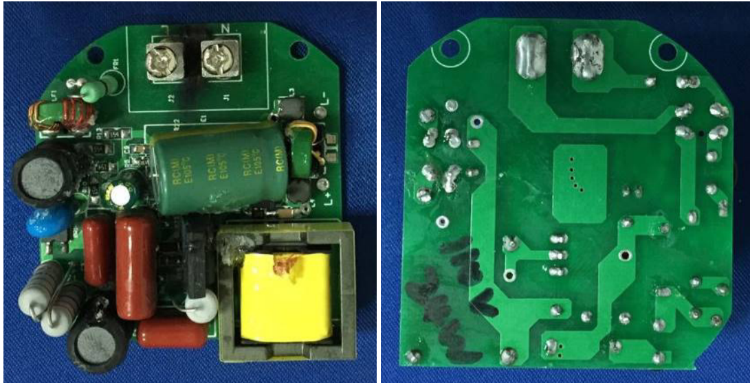
Picture 7. model: B0104-24-Y-3-Z LED driver view
