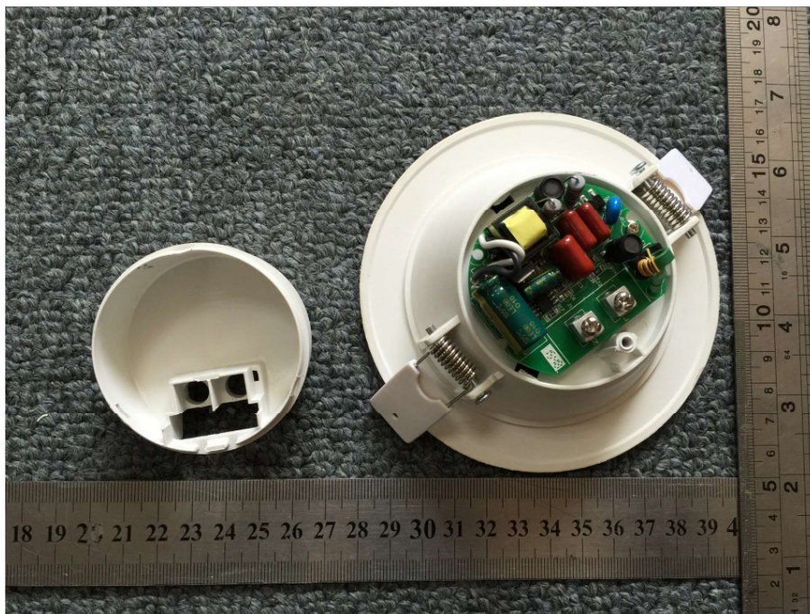
Picture 18. model: B0104-12-Y-1-Z, B0104-12-Y-3-Z internal view (II)
