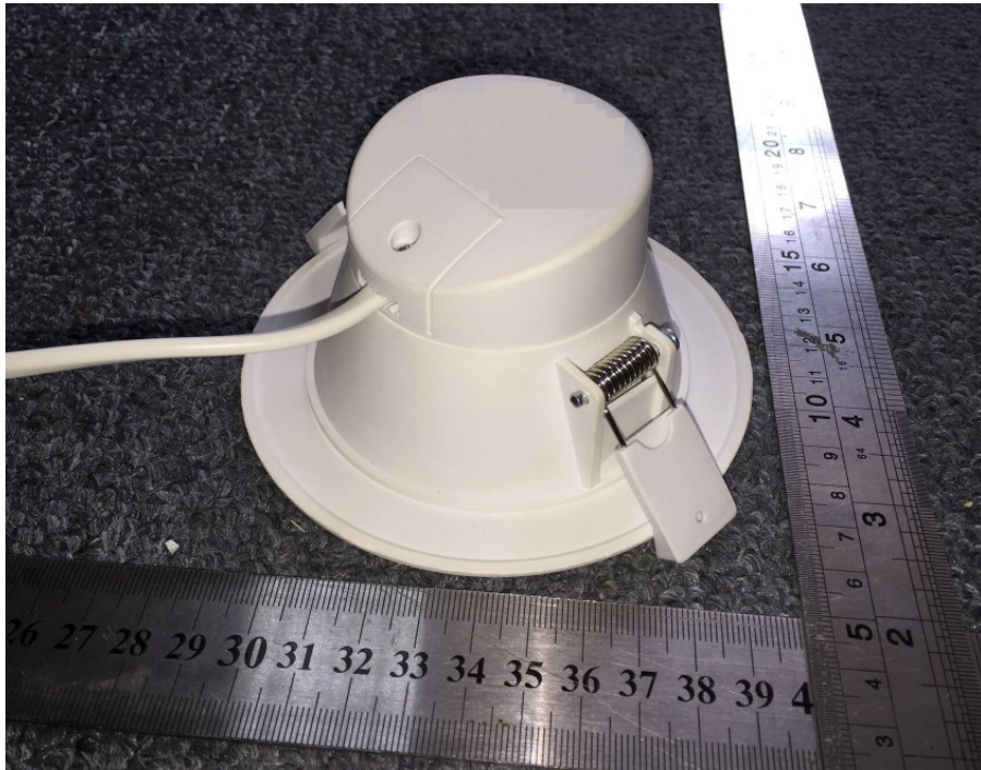
Picture 16. model: B0104-12-Y-1-Z, B0104-12-Y-3-Z bottom view
