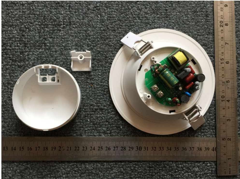
Picture 11. model: B0104-15-Y-1-Z, B0104-15-Y-3-Z internal view (II)
