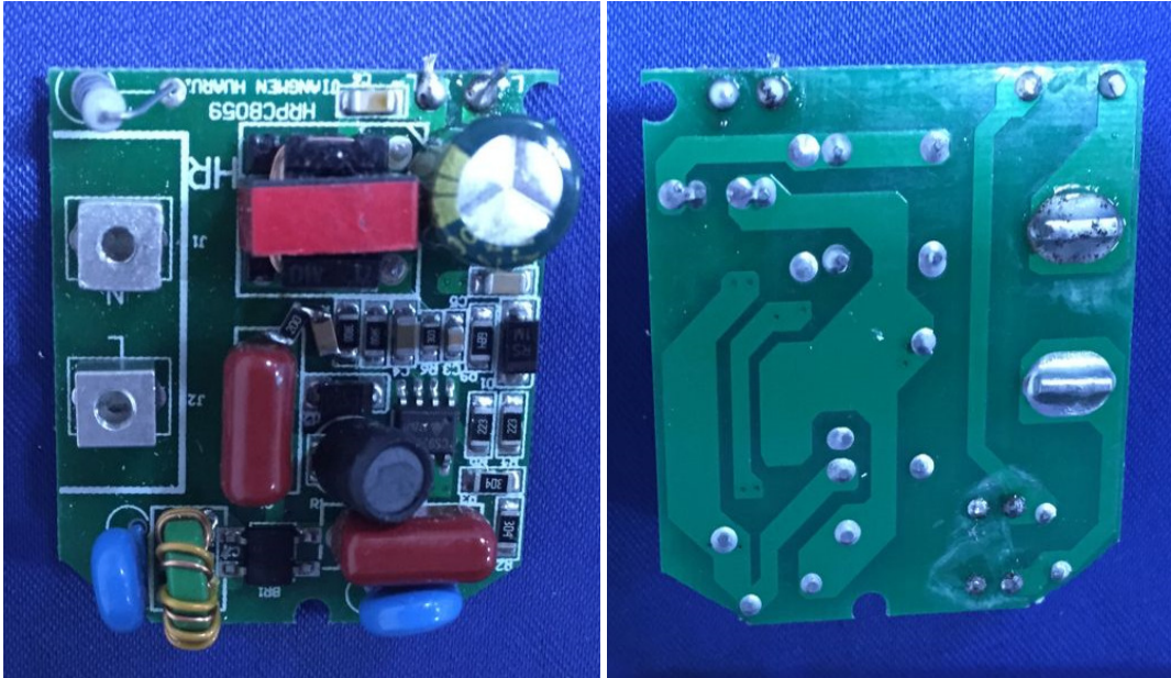
Picture 20. model: B0104-12-Y-1-Z LED driver view
