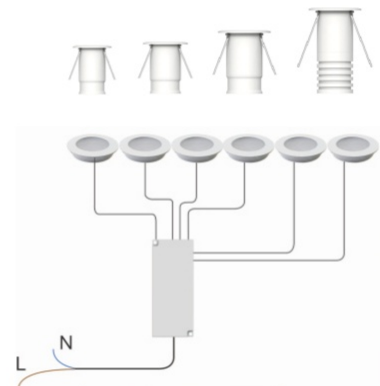
Connect to 110V or 230V
